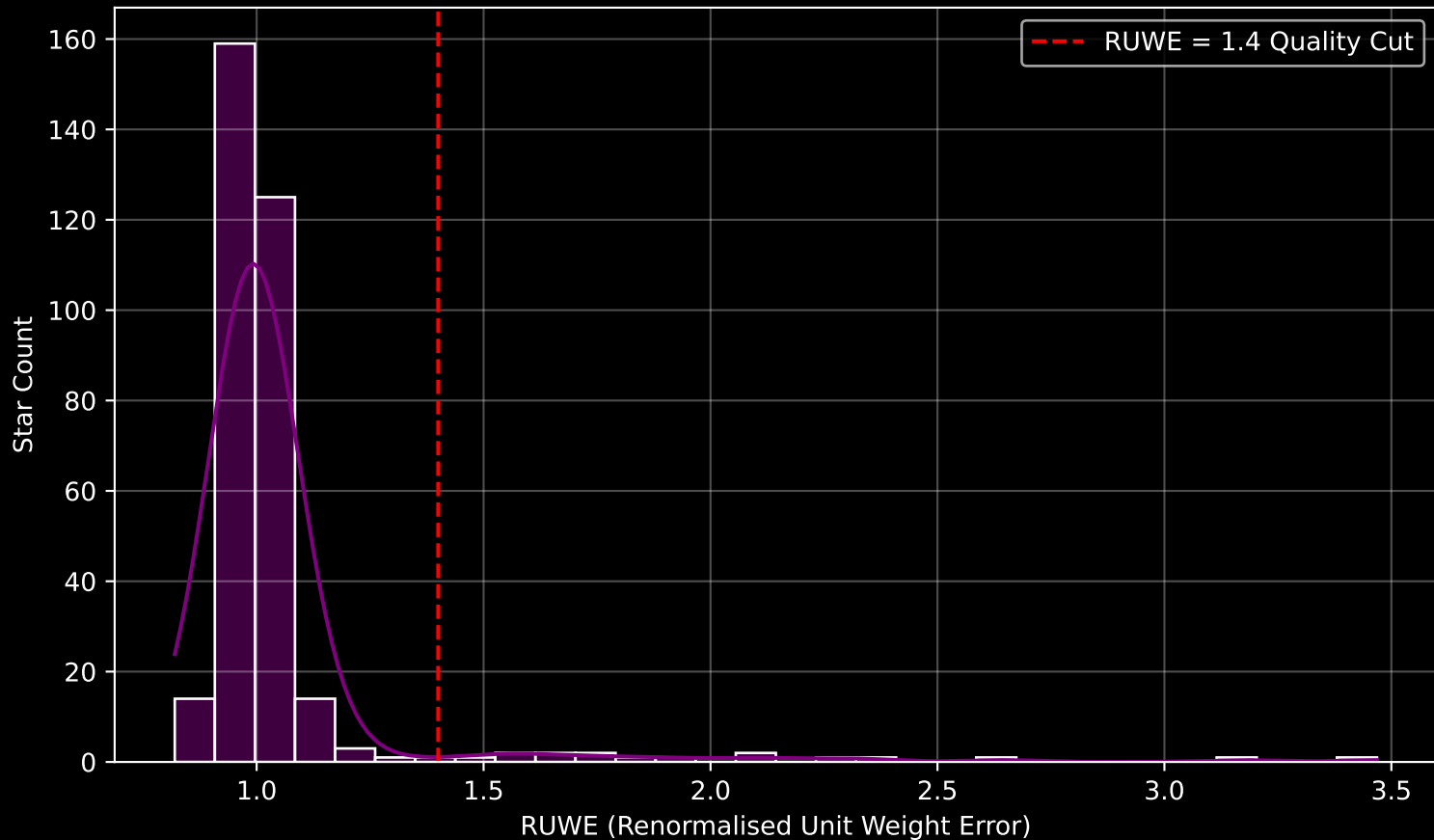
GAPOGEE DR17 Field [M71_btx] RUWE Distribution (n= 333)
