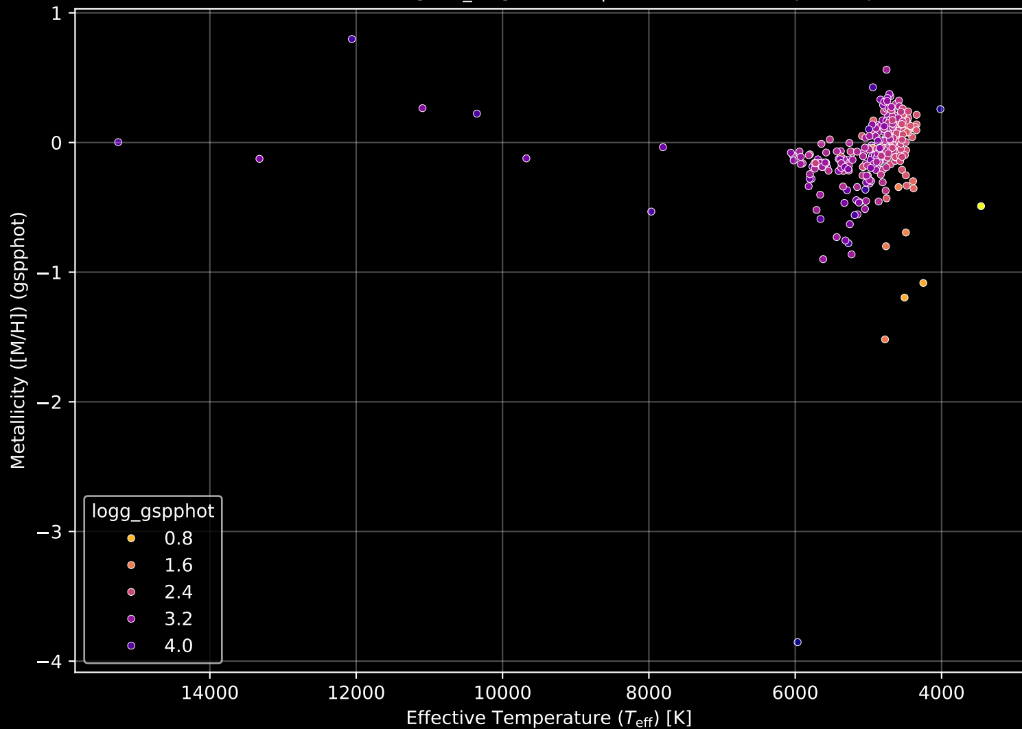
APOGEE DR17 Field: [M71_btx] Stellar Population Parameters (n= 333)
