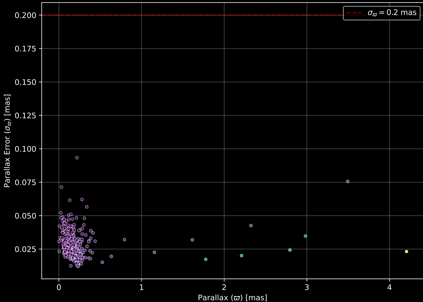
APOGEE DR17 Field: [M71_btx] Parallax Quality (n= 333)
