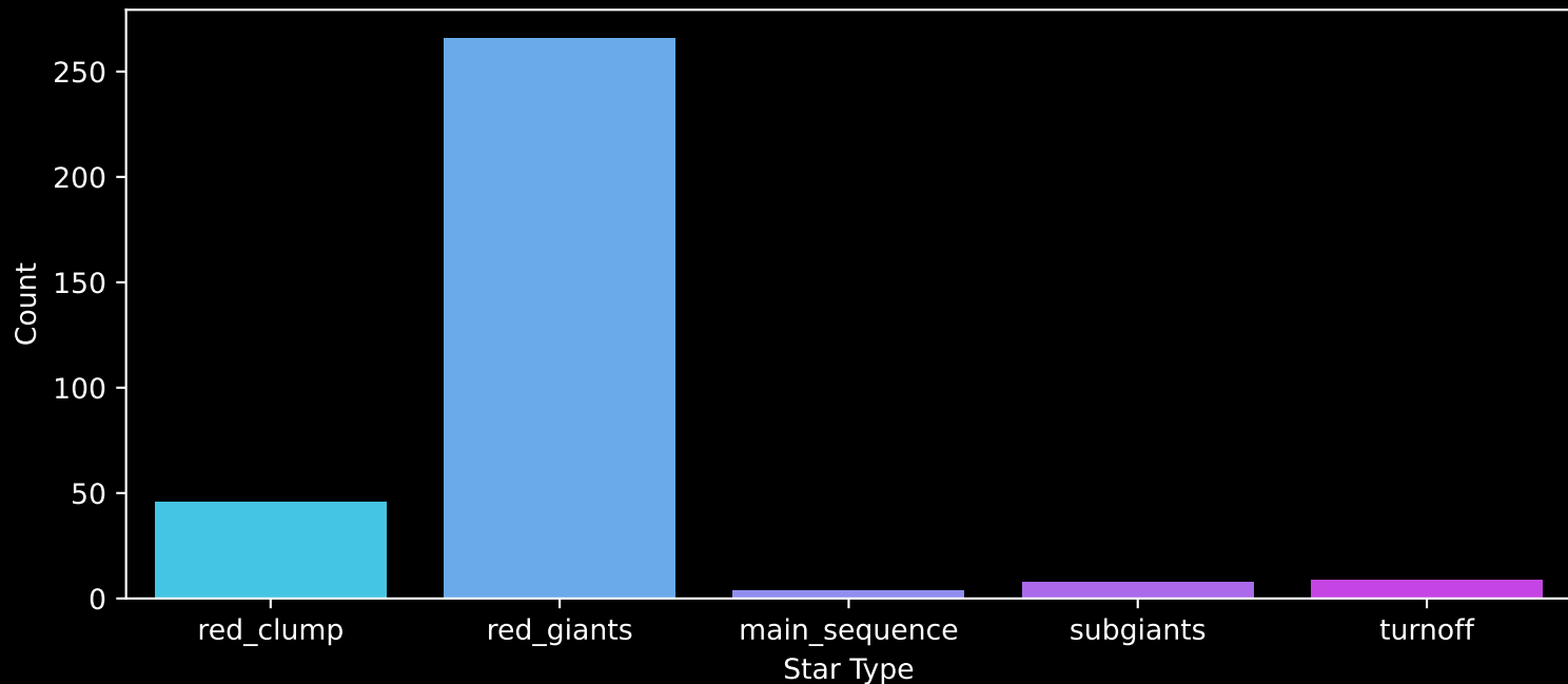
APOGEE DR17 Field: [M71_btx] Count plot of Star Type
