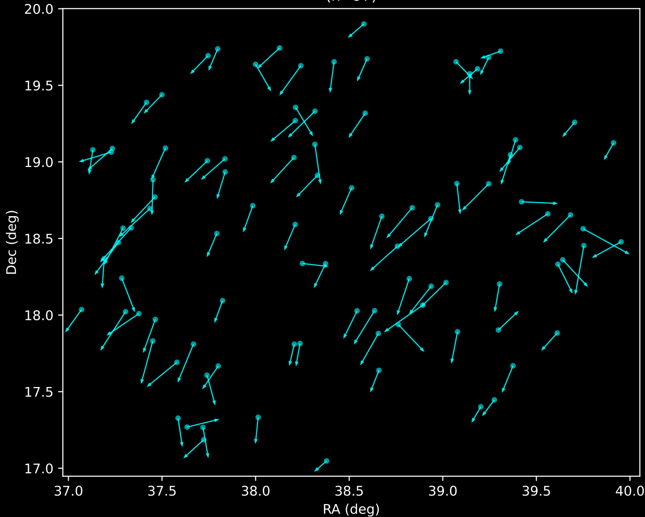
APOGEE DR17 Noise Stream Proper Motion Vectors (n=97)
