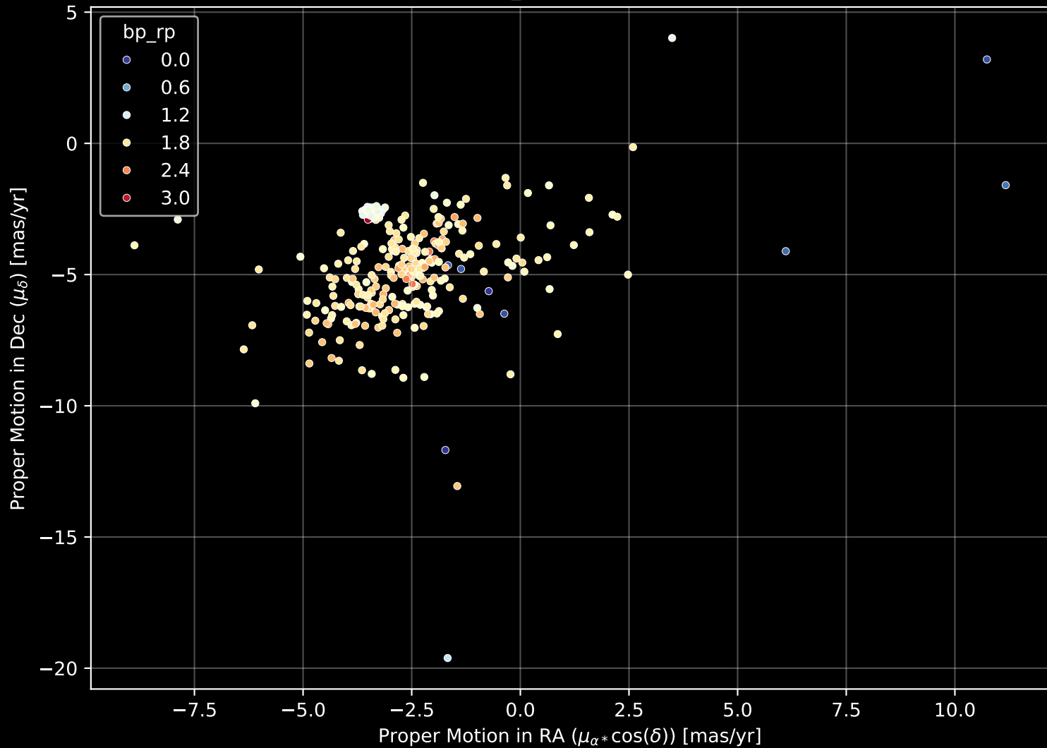
APOGEE DR17 Field: [M71_btx] Proper Motion Diagram (n= 333)
