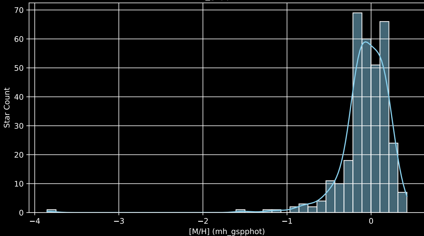
APOGEE DR17 Field: [M71_btx [M/H] (mh_gspphot) (n= 331)
